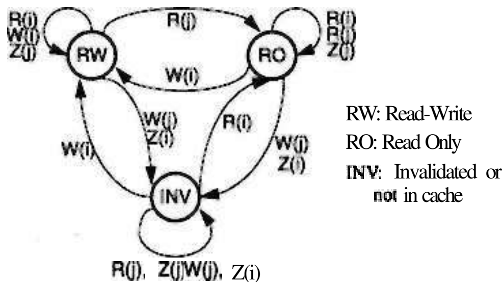
(a) Write-through cache
