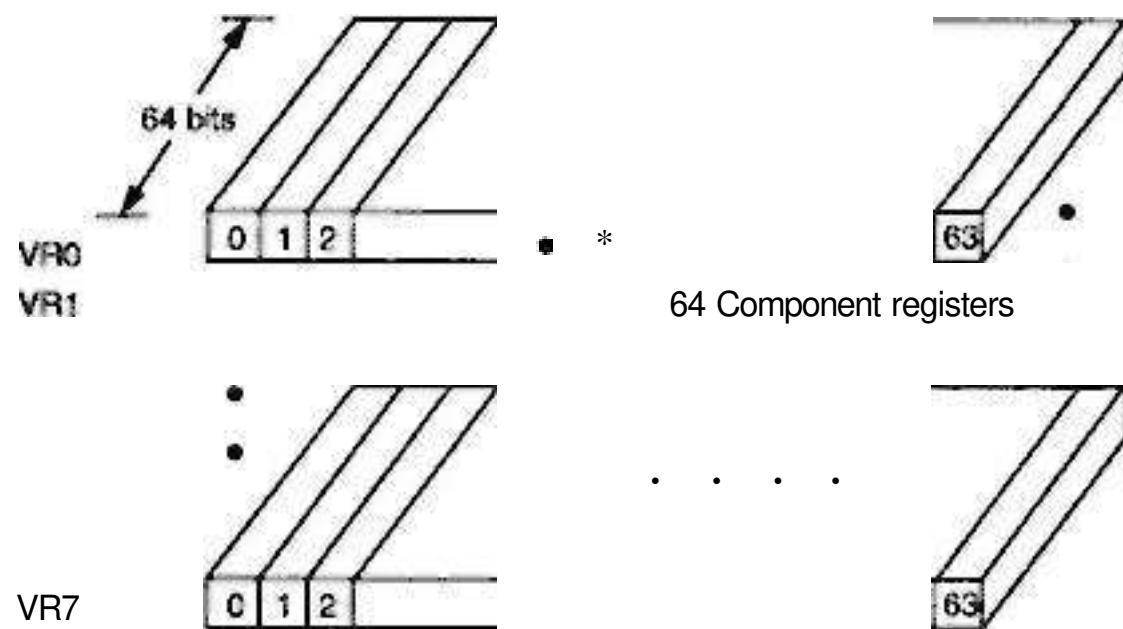
(a) Eight vector registers (8 x 64 x 64 bits) on Cray machines
