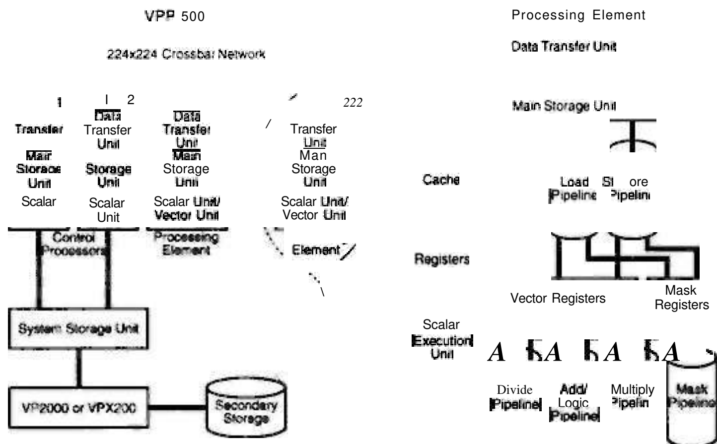
Figure 8.15 The Fujitsu VPP500 architecture. (Courtesy of Fujitsu Ltd., 1992)
