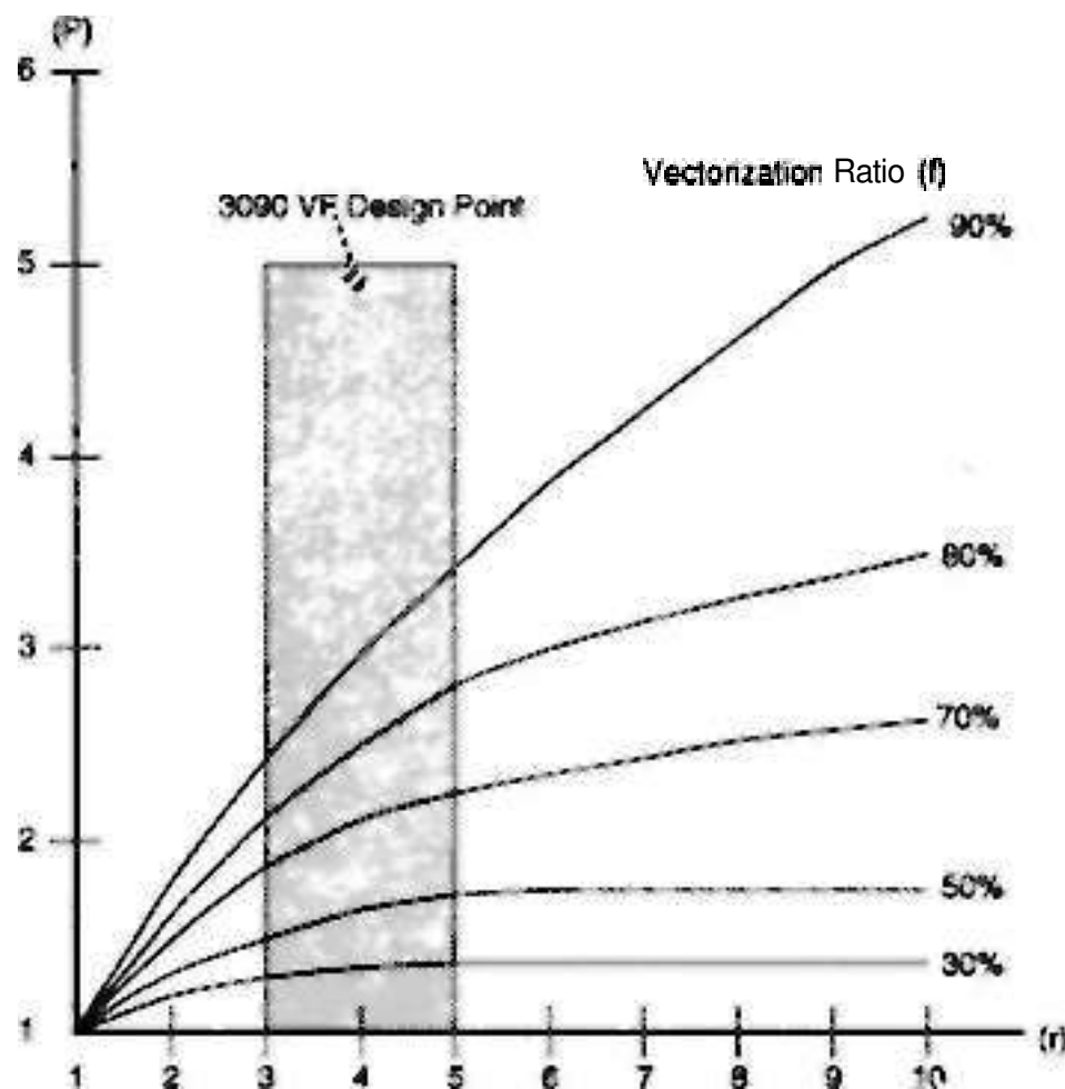
Figure 8.6 Speedup performance of vector processing over scalar processing in the IBM 3090/VF. (Courtesy of IBM Corporation, 1986)
