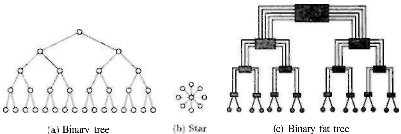
Figure 2.17 Tree , star, and fat tree.
