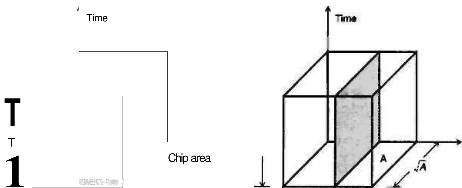
(a) Memory-limited bound on chip area A and I/O-limited bound on chip history represented by the volume AT
