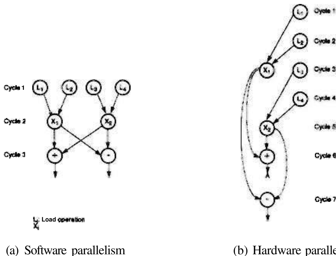
Figure 2.3 Executing an example program by a two-issue superscalar processor.
