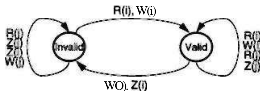
(a) Write-through cache
