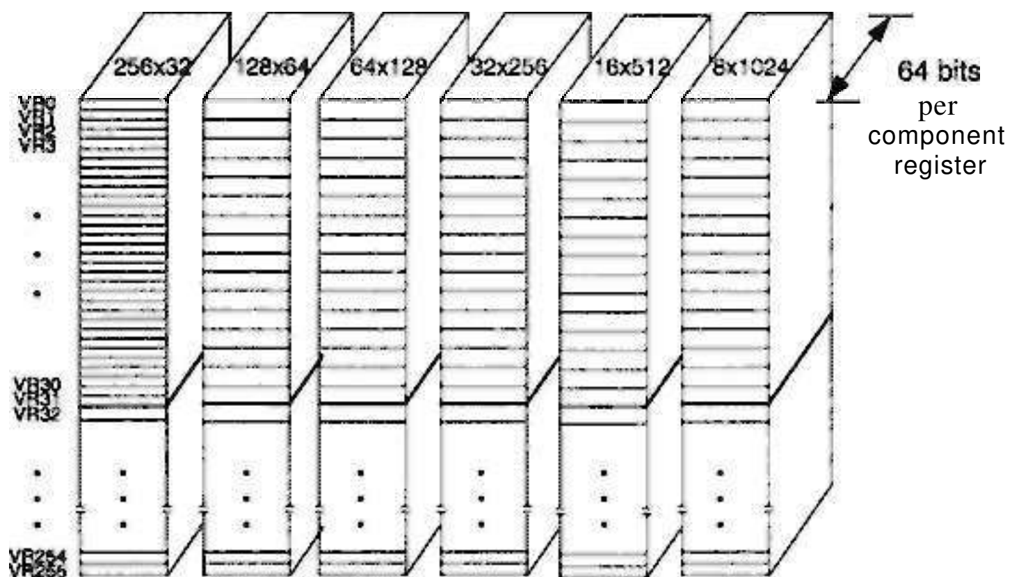
(b) Vector register configurations in the Fujitsu VP2000
