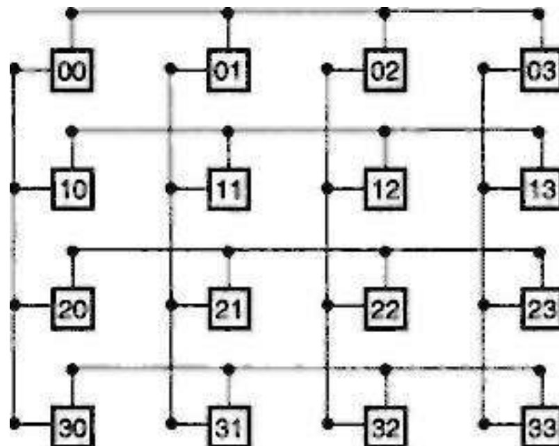
Figure 1.16 A 4x4 mesh of processing elements (PEs) with broadcast buses on each row and on each column. (Courtesy of Prasanna Kumar and Raghavendra; reprinted from Journal of Parallel and Distributed Computing , April 1987)
