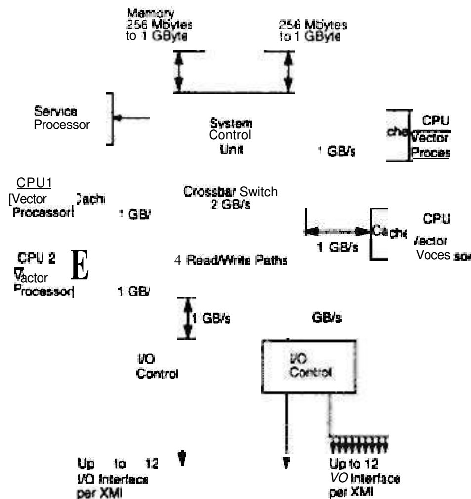
(a) The VAX 9000 multiprocessor system
