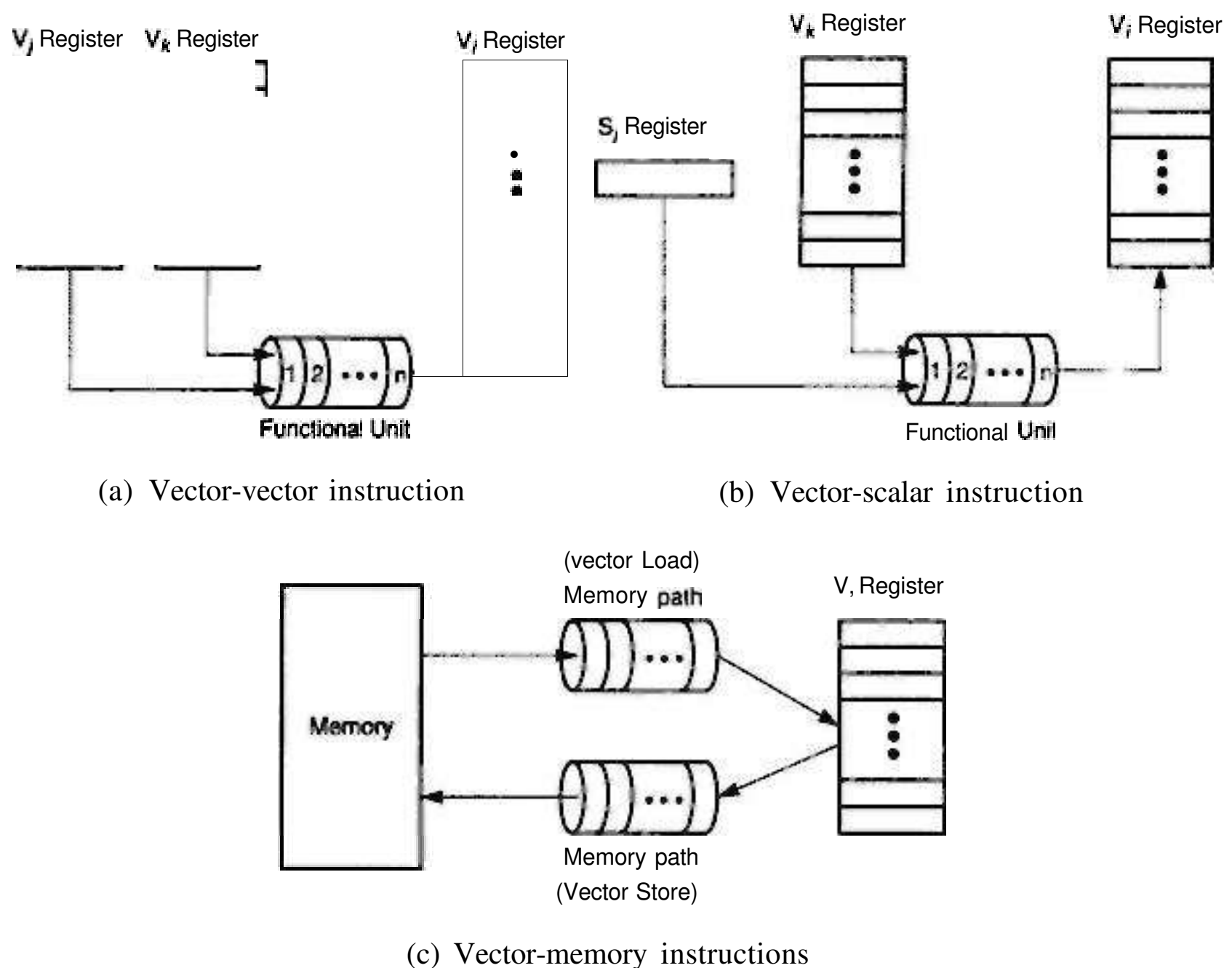
Figure 8.1 Vector instruction types in Cray-like computers.
