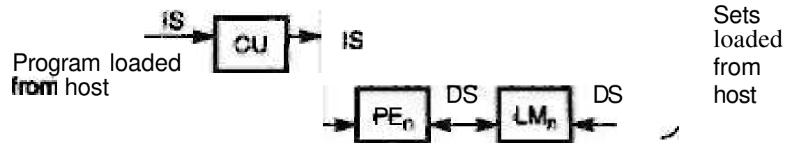
(b) SIMD architecture (with distributed memory)
