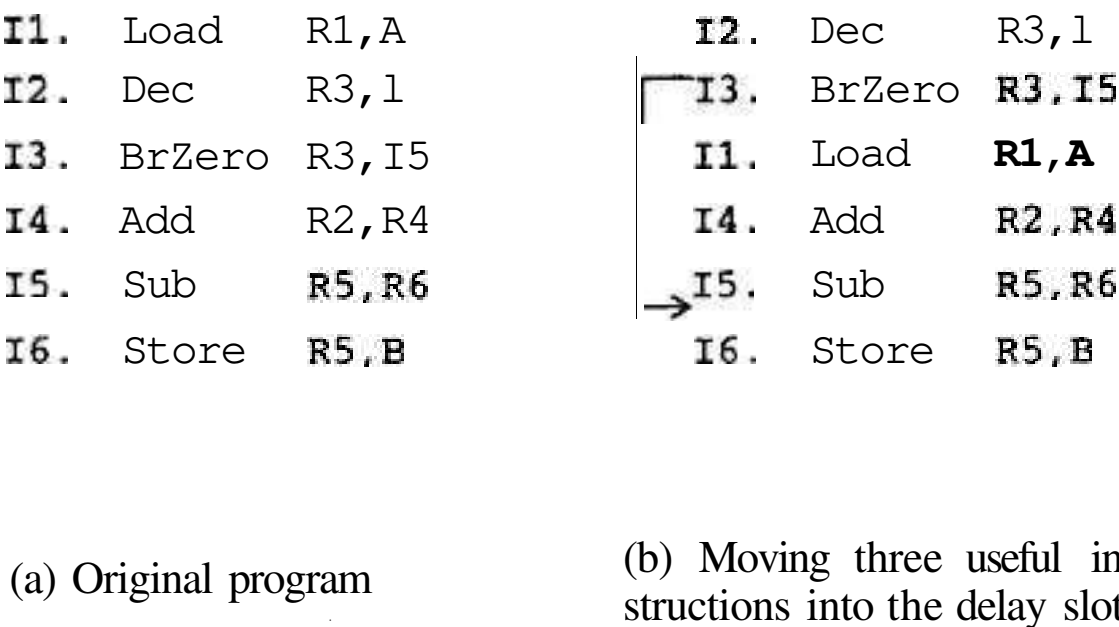
Figure 6.21 Code motion across a branch to achieve a delayed branch with a re- duced penalty to pipeline performance.
