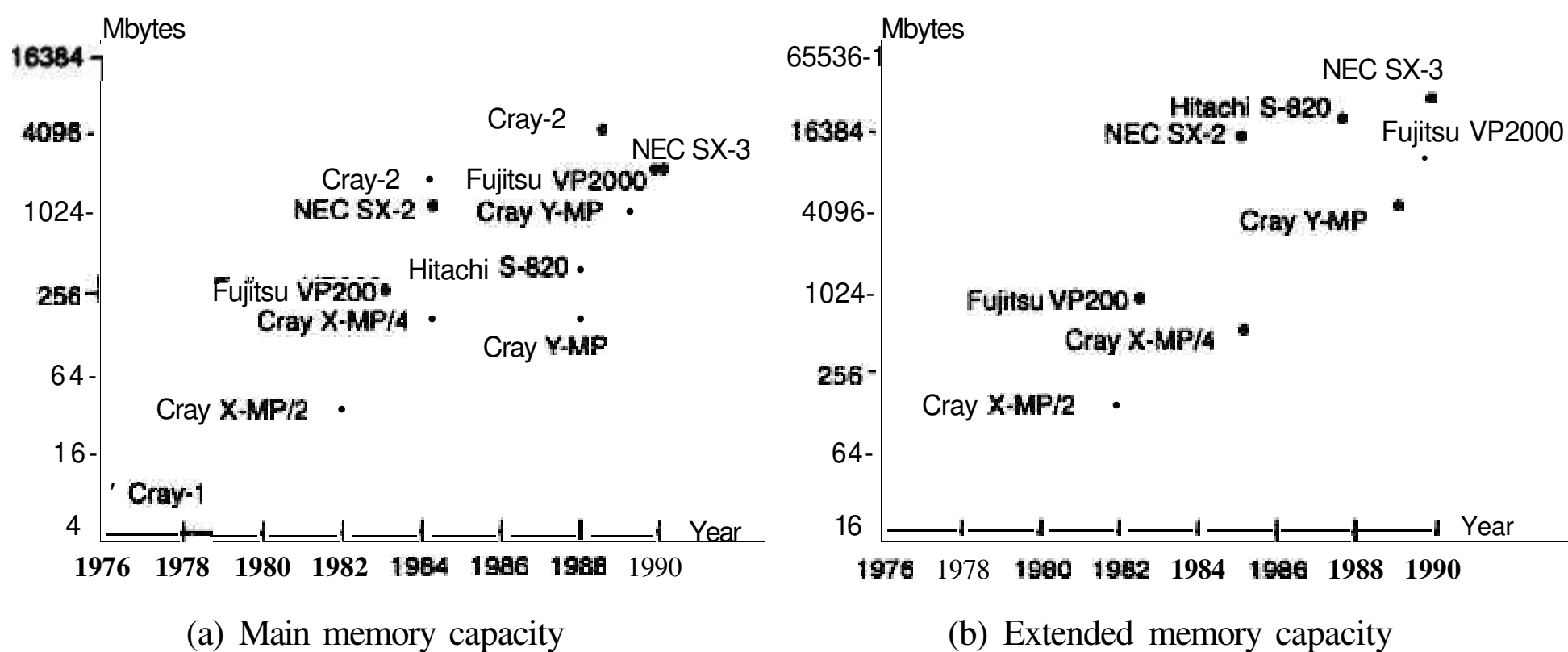
Figure 8.8 Supercomputer memory capacities (Source: Smith, Hsu, and Hsiung, IEEE Supercomputing Conference , 1990)
