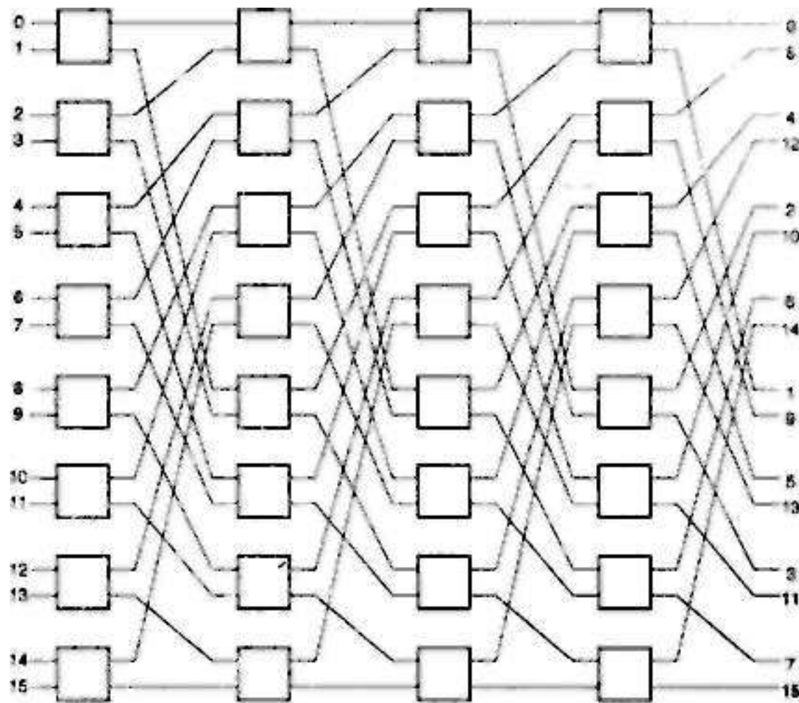
Figure 2.27 A 16 x 16 Flip network. (Courtesy of Ken Batcher; reprinted from Proc. Int. Conf. Parallel Processing , 1976)
