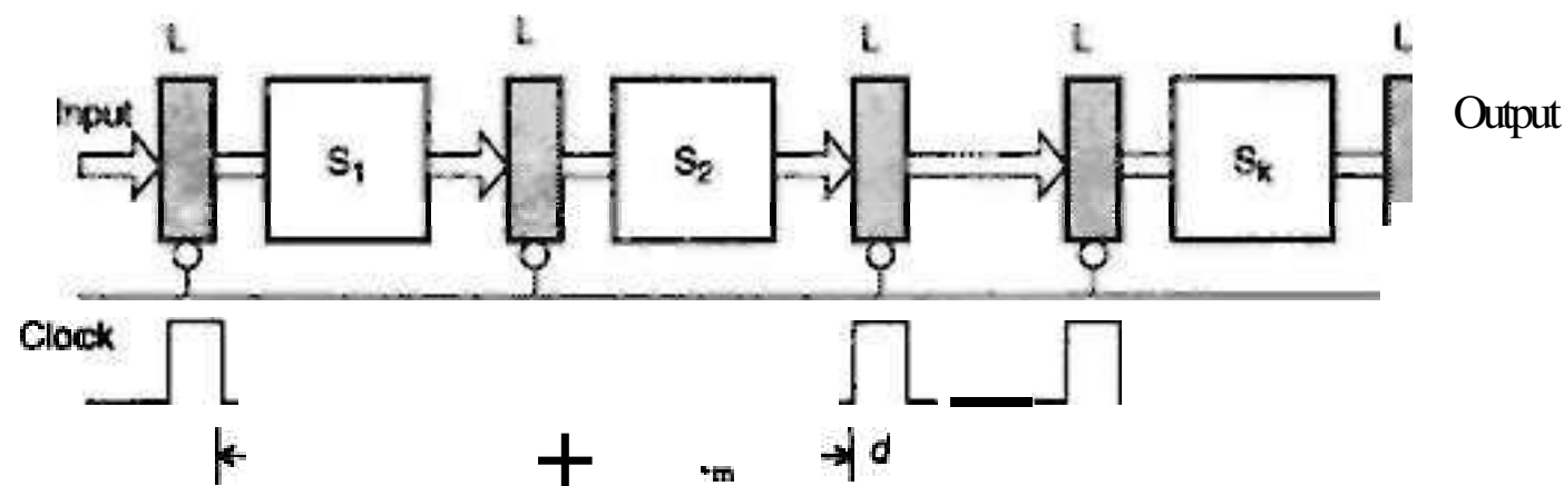
(b) A synchronous pipeline model
