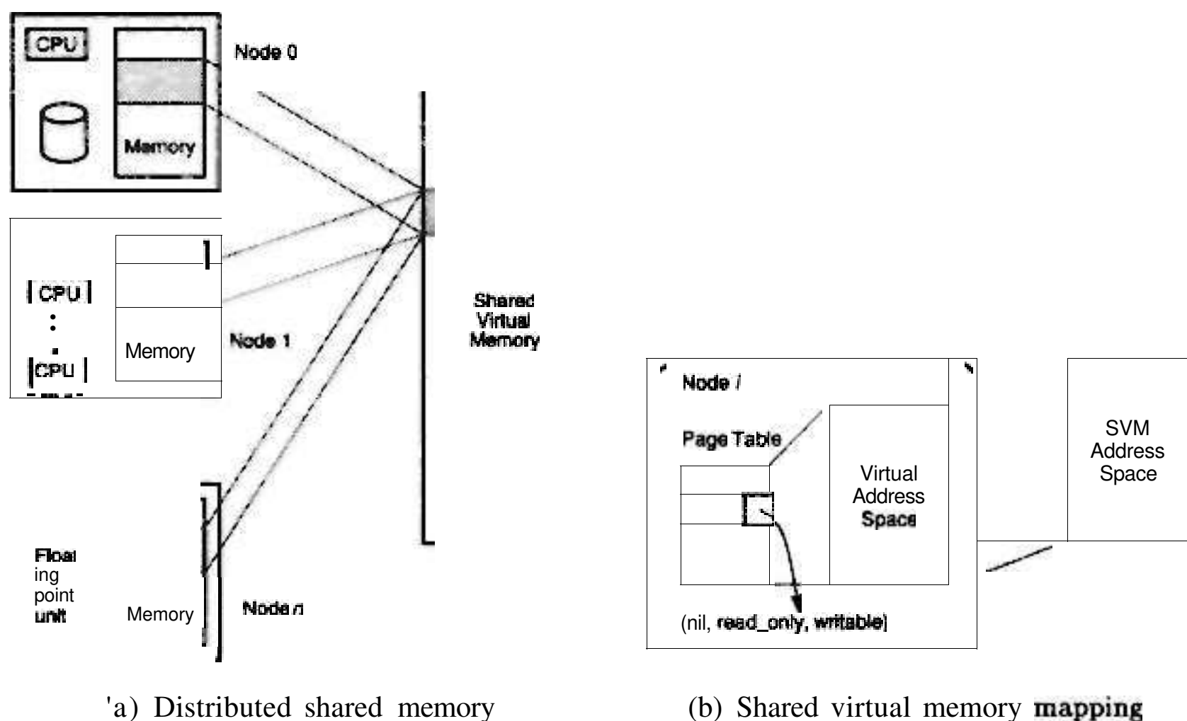
Figure 9.2 The concept of distributed shared memory with a global virtual address space shared among all processors on loosely coupled processing nodes in a massively parallel architecture. (Courtesy of Kai Li, 1992)
