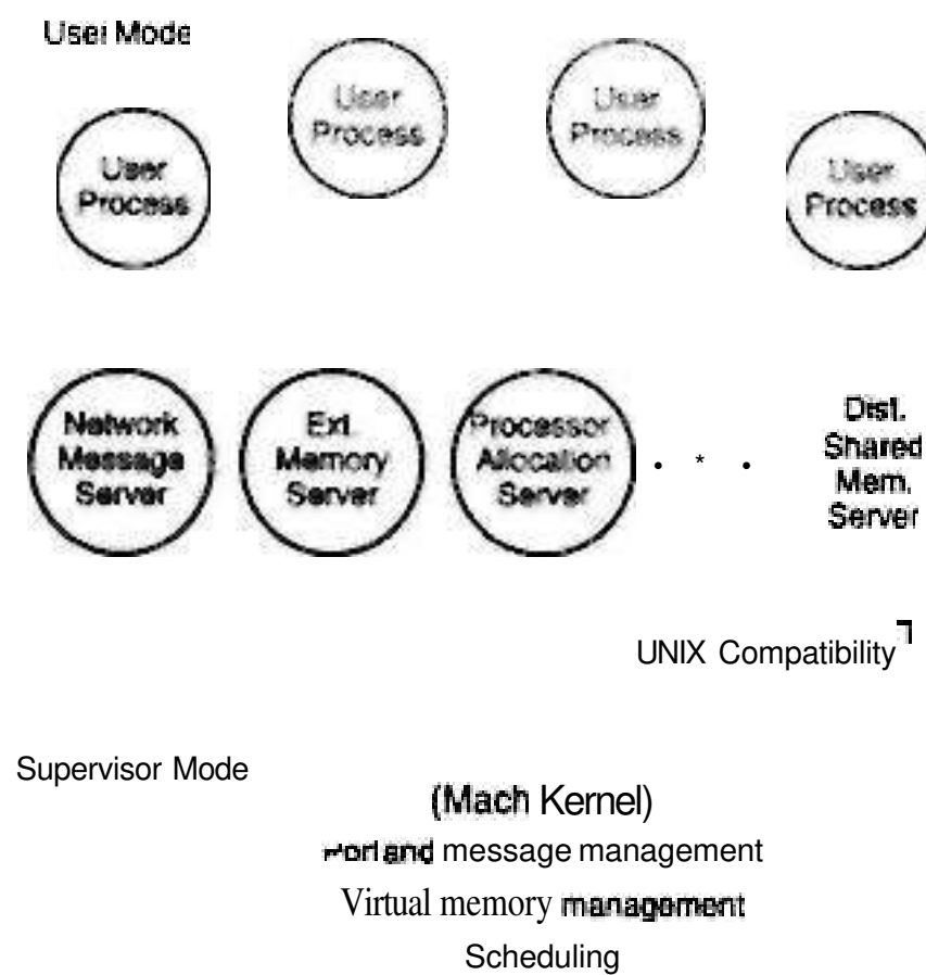
Figure 12.10 The Mach/OS kernel and various user-level servers with UNIX compatibility ,
