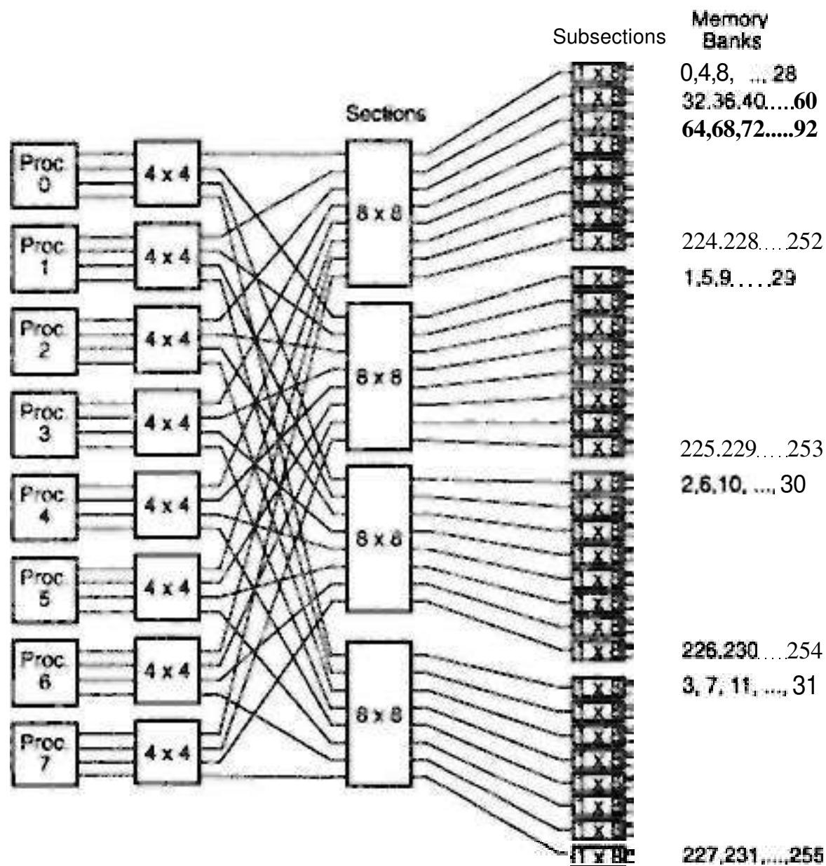
Figure 8.10 Schematic logic diagram of the crossbar network between 8 processors and 256 memory banks in the Cray Y-MP 816.
