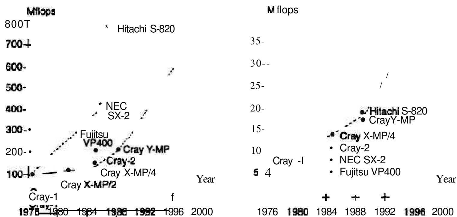
(a) Uniprocessor vector performance
