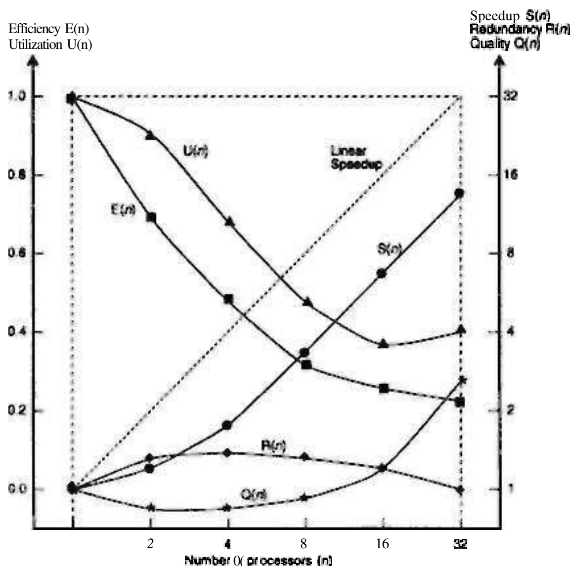
Figure 3.4 Performance measures for Example 3.3 on a parallel computer with up to 32 processors.
