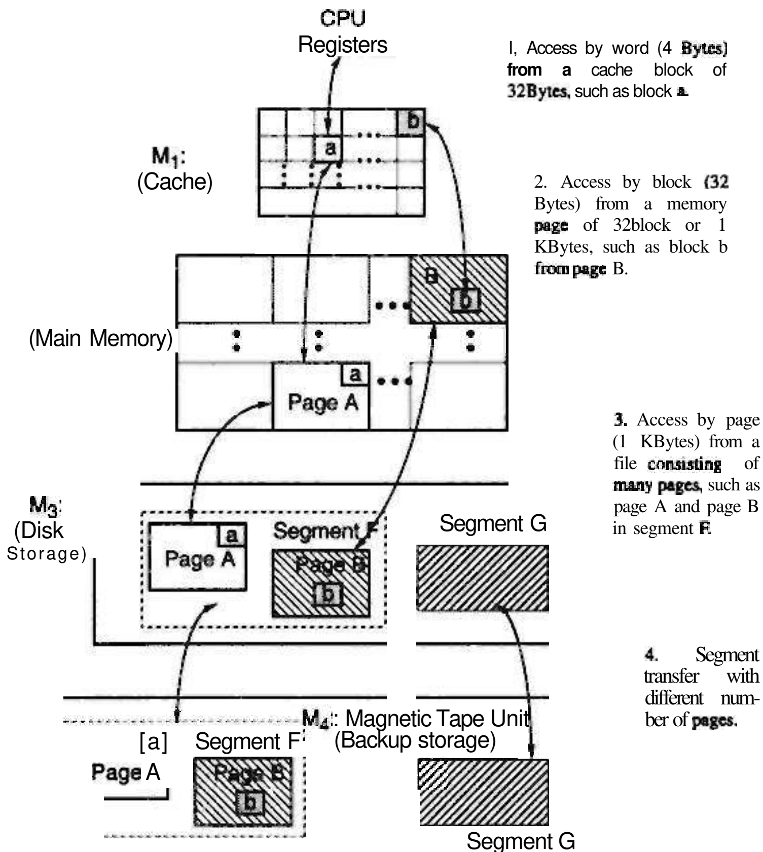
Figure 4.18 The inclusion property and data transfers between adjacent levels of a memory hierarchy.
