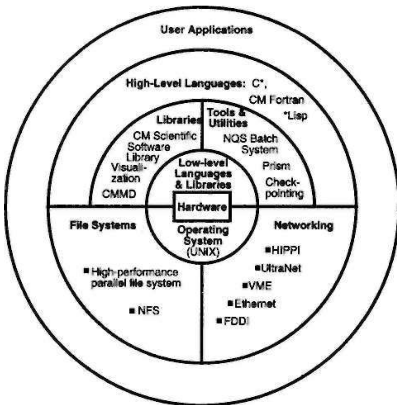
Figure 11.3 Software layers of the Connection Machine system. (Courtesy of Thinking Machines Corporation, 1992)
